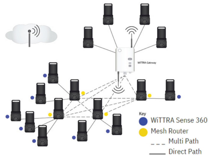
Combined (6LoWPAN + LPWAN)
